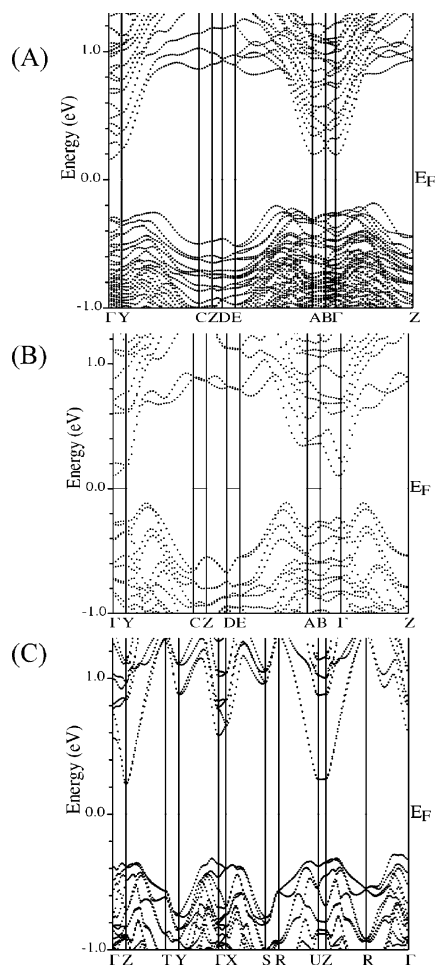
Figure 2. Band structure plots of (a) \alpha -RbBi 3 Se 5 ( E_g = 0.39 eV), (b) \beta -RbBi 3 Se 5 ( E_g = 0.22 eV), and (c) \gamma -RbBi 3 Se 5 ( E_g = 0.56 eV). Monoclinic symmetry ( \alpha , \beta ) points: \Gamma = (0,0,0) ; Y = (0,0.5,0); C = (0,0.5,0.5); Z = (0,0,0.5); D = (0.5,0,0.5); E = (0.5,-0.5,0.5); A = (0.5,-0.5,0); B = (0.5,0,0). Orthorhombic symmetry (Y) points: \Gamma = (0,0,0) ; Z = (0,0,0.5); T = (0,0.5,0.5); Y = (0,0.5,0); X = (0.5,0,0); S = (0.5,0.5,0); R = (0.5,0.5,0.5); U = (0.5,0,0.5).
