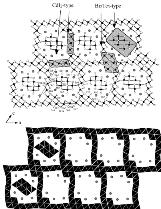
Figure 5. Projection of the structure of \alpha - RbBi_3Se_5 down the b -axis (top). The shaded areas indicate the Bi 2 Te 3 - and CdI 2 -type building blocks. Polyhedral representation of the structure of \alpha - RbBi_3Se_5 (bottom). Most of the Bi 2 Te 3 -type fragments has been removed to show the large rectangular tunnels.
