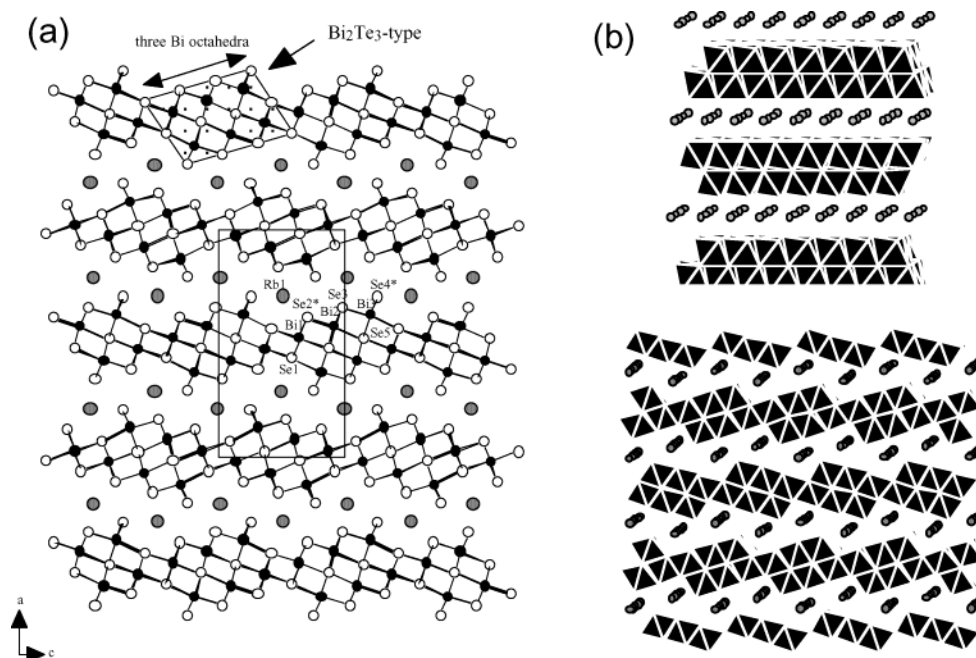
Figure 7. (a) Projection of the structure of \gamma - \text{RbBi}_3\text{Se}_5 (also adopted by \text{RbBi}_3\text{Se}_4\text{Te} ) down the b -axis. The shaded area indicates the \text{Bi}_2\text{Te}_3 -type building block, and the (*)'s indicate the Te containing chalcogen sites in \text{RbBi}_3\text{Se}_4\text{Te} . (b) Polyhedral representation of the structures of \text{RbPbBi}_3\text{Se}_6 (top) and \gamma - \text{RbBi}_3\text{Se}_5 (bottom).
