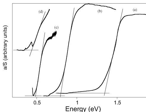
Figure 1. Solid-state UV/vis and infrared absorption spectra showing band-gap transitions for (a) \gamma - RbBi_3S_5 (b) \gamma - RbBi_3Se_5 , (c) \beta - RbBi_3Se_5 , and (d) \alpha - RbBi_3Se_5 . The band gaps in each case are estimated from the crossing point of the solid lines shown in each spectrum.
