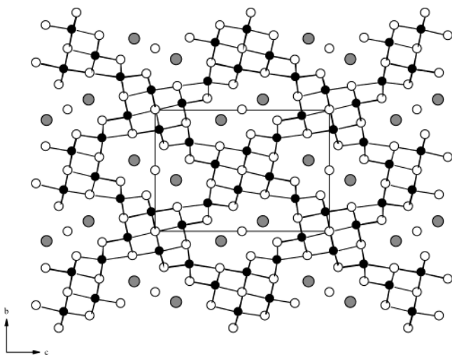
Figure 4. Projection of the structure of \alpha - RbBi_3S_5 down the a -axis. Adapted using atomic coordinates reported in ref 15f.
